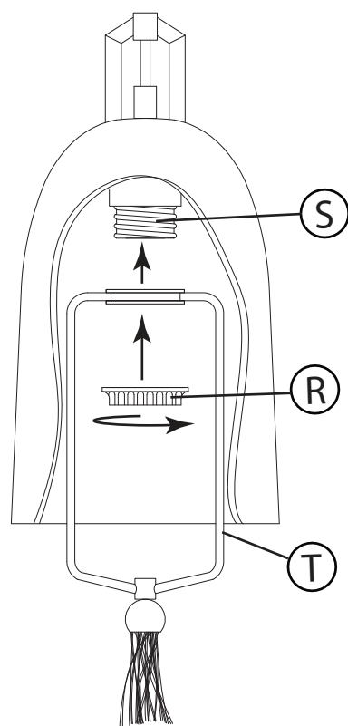
DRAWING 2 - ASSEMBLY
