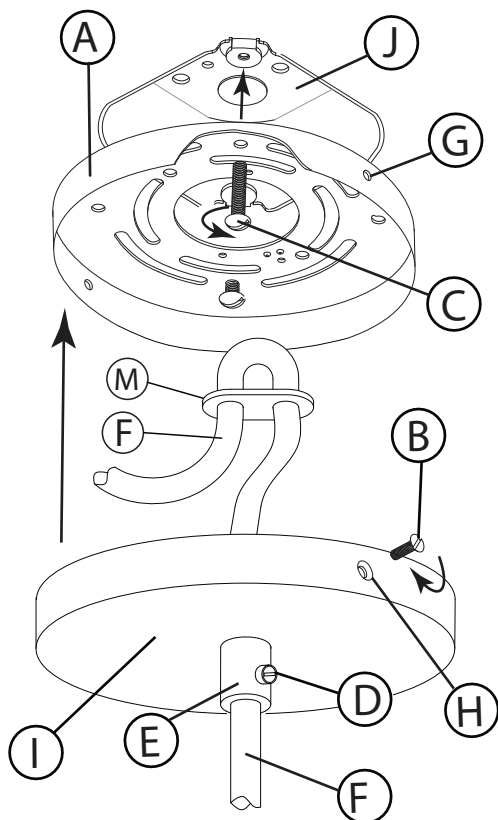
DRAWING 2 - ASSEMBLY
